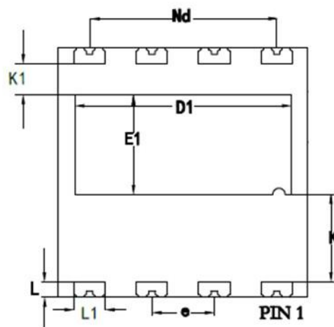
BOTGOM VIEW
