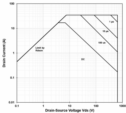
Figure 18 Safe Operation Area
