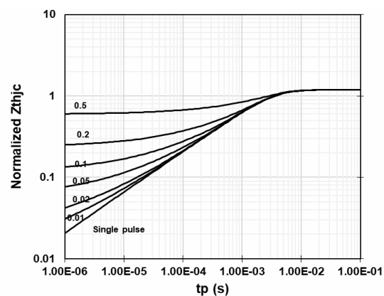
Figure 17 Max.transient thermal impedance
