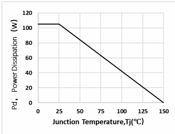
Figure 16 Power dissipation
