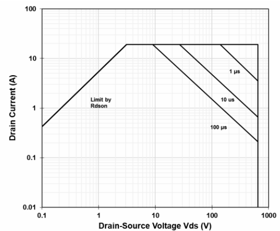
Figure 19 Safe Operation Area
