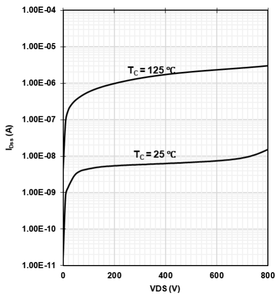
Figure 9 Drain-source leakage characteristics
