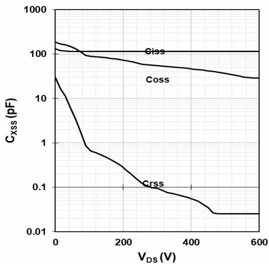
Figure 10 Typ. capacitances
