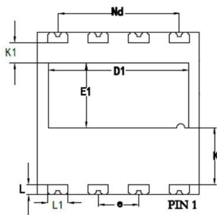
BOTGOM VIEW
